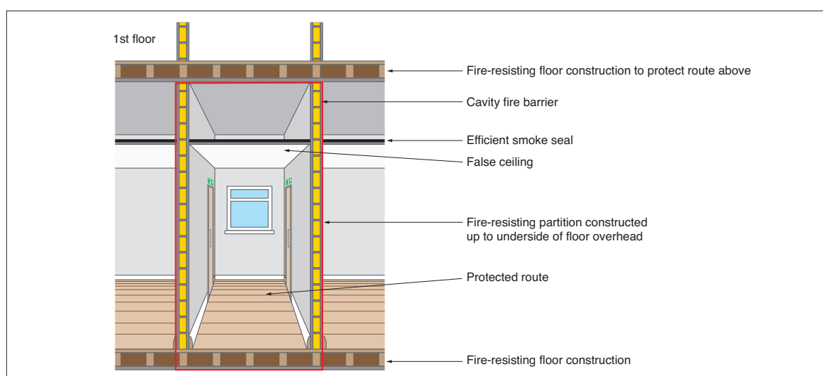
Figure 31: Fire-resisting construction
