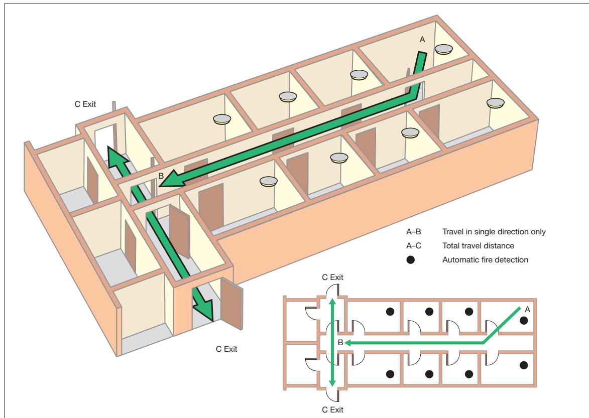
Figure 29: Dead-end condition with automatic fire detection
