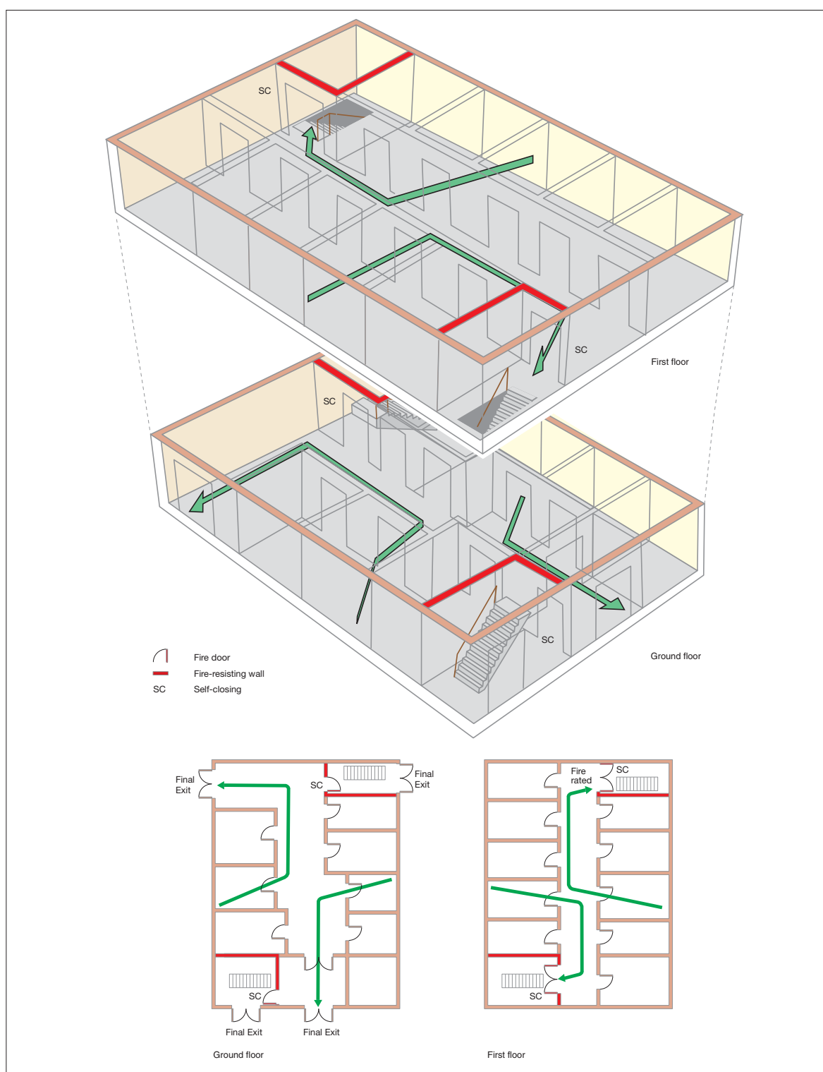
Figure 45: Two-storey, ground and one upper floor
