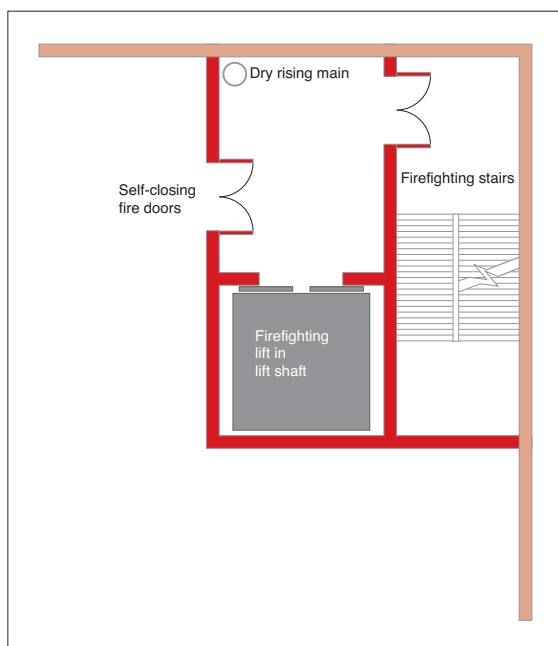
Figure 19: Firefighting shaft
